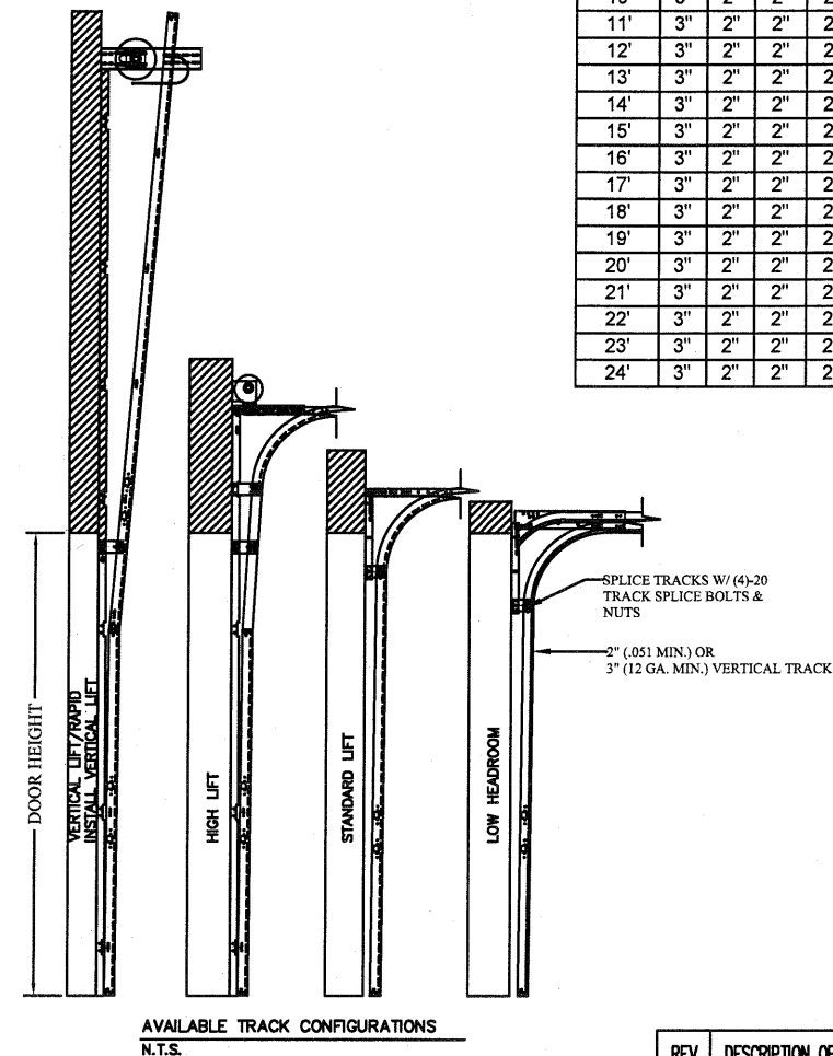
DOOR HEIGHT A B C D E F G H I J K L M N O P Q R S SPACING S 7' 10" 34" 58" 76" 8' 10" 34" 58" 88" 9' 10" 34" 58" 82" 100" 10' 10" 34" 58" 82" 94" 112" 11' 10" 34" 58" 82" 94" 106" 124" 12' 10" 34" 58" 82" 94" 106" 118" 136" 13' 10" 34" 58" 82" 94" 106" 118" 130" 148" 14' 10" 34" 58" 82" 94" 106" 118" 130" 142" 160" 15' 10" 34" 58" 82" 94" 106" 118" 130" 142" 154" 172" 16' 10" 34" 58" 82" 94" 106" 118" 130" 142" 154" 166" 184" 17' 10" 34" 58" 82" 94" 106" 118" 130" 142" 154" 166" 178" 196" 18' 10" 34" 58" 82" 94" 106" 118" 130" 142" 154" 166" 178" 190" 208" 19' 10" 34" 58" 82" 94" 106" 118" 130" 142" 154" 166" 178" 190" 202" 220" 20' 10" 34" 58" 82" 94" 106" 118" 130" 142" 154" 166" 178" 190" 202" 214" 232" 21' 10" 34" 58" 82" 94" 106" 118" 130" 142" 154" 166" 178" 190" 202" 214" 226" 244" 22' 10" 34" 58" 82" 94" 106" 118" 130" 142" 154" 166" 178" 190" 202" 214" 226" 238" 256" 23' 10" 34" 58" 82" 94" 106" 118" 130" 142" 154" 166" 178" 190" 202" 214" 226" 238" 250" 268" 24' 10" 34" 58" 82" 94" 106" 118" 130" 142" 154" 166" 178" 190" 202" 214" 226" 238" 250" 262" 280"
